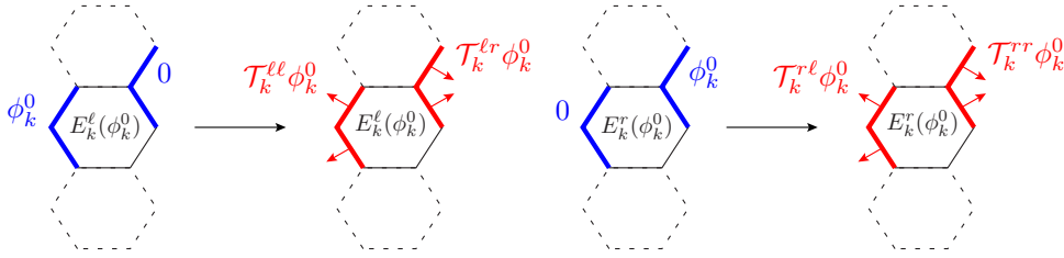
FIG. 5.5. The four local DtN operators
