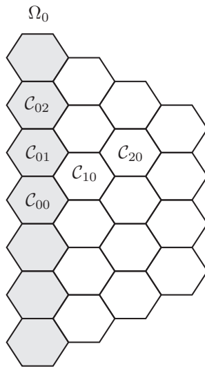
FIG. 2.3. Description of the half-space \Omega^H and its periodicity cells
