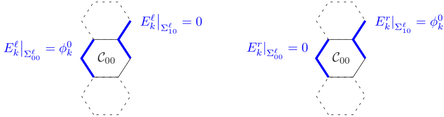
FIG. 5.4. The two strip problems for E_k^\ell (on the left) and E_k^r (on the right)
