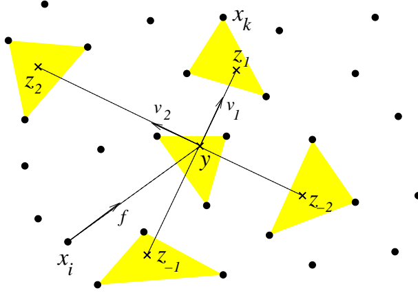
Figure 1. Construction of the MDP approximation scheme. Here q = n = 2 .
